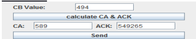
Fig 7.1 User calculating c_A and ACK
